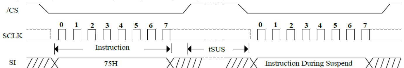
Figure37. Erase/Program Suspend Command Sequence
